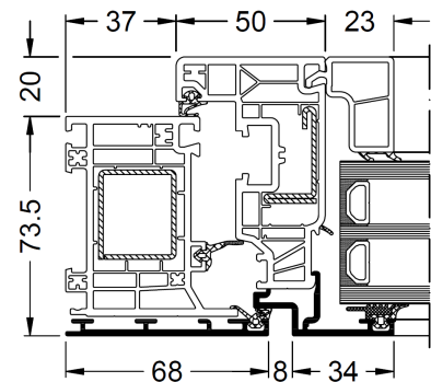
Schüco Symbiotic Design
