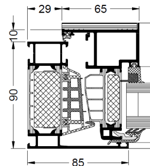
AWS 90 BS.SI+ WoodDesign
